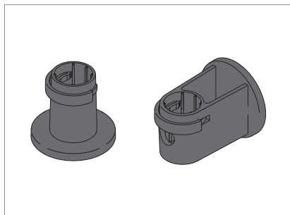
Fig. 5: Adaptor models.
